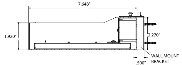
Wall Mount Dimensions
