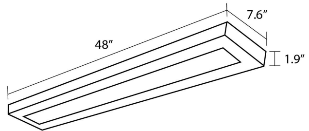
Wall Mount Dimensions
