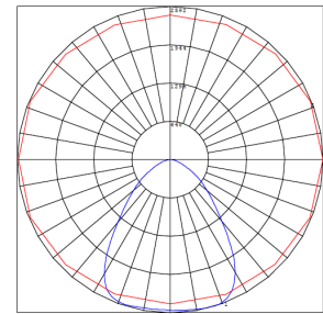
BUG Rating: B3-U0-G1
