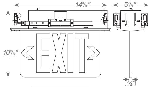
Recessed Wall
