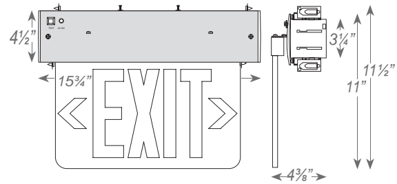
Recessed Wall
