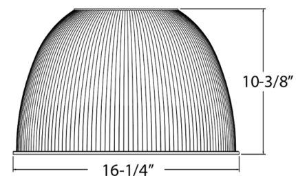
Prismatic polycarbonate refractor shade (CPR)
