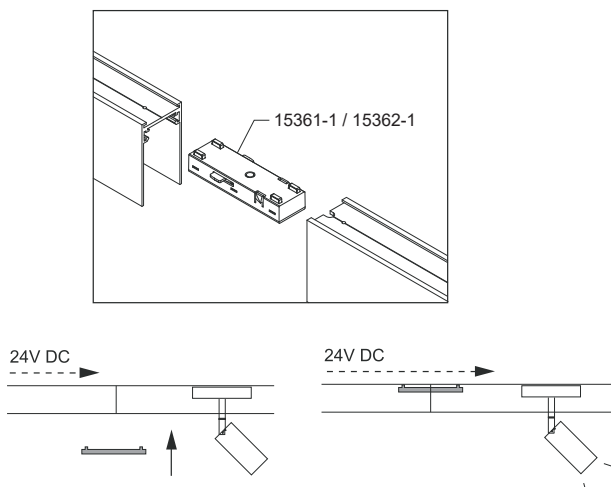
Using circuit joint (15361-1 / 15362-1) to connect between tracks
