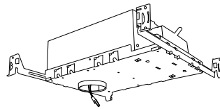
2" IC Airtight Construction Housing Height: 4" Opening: 2 1/2"
