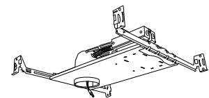
2" Non-IC Construction Housing Height: 3 1/2" Opening: 2 1/2"
