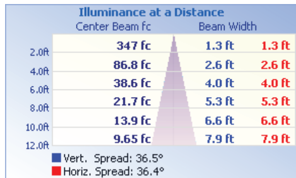
Cone of Light based on mounting height of 12'
