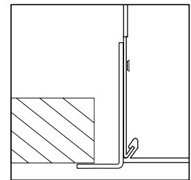
RF - Flange Detail
