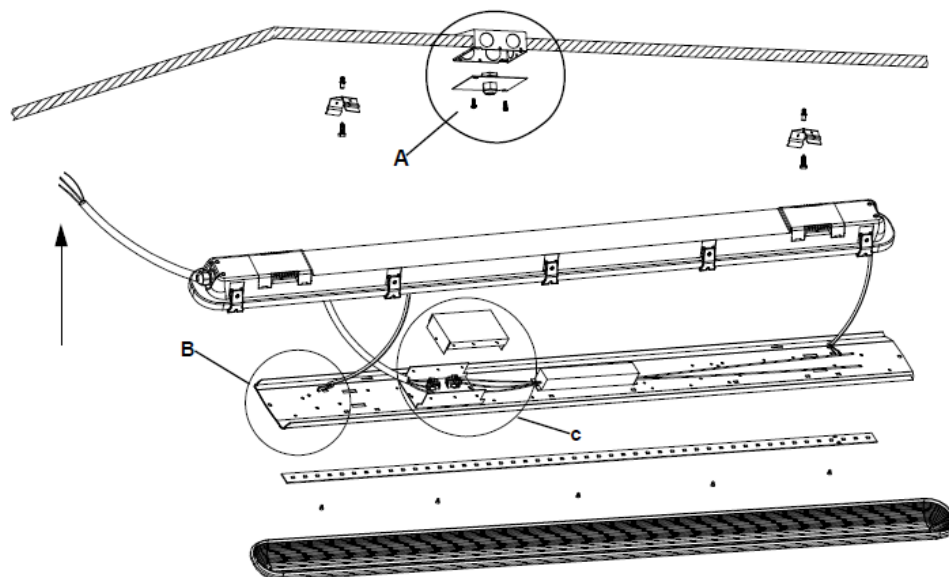
Surface Ceiling Mount Diagram
