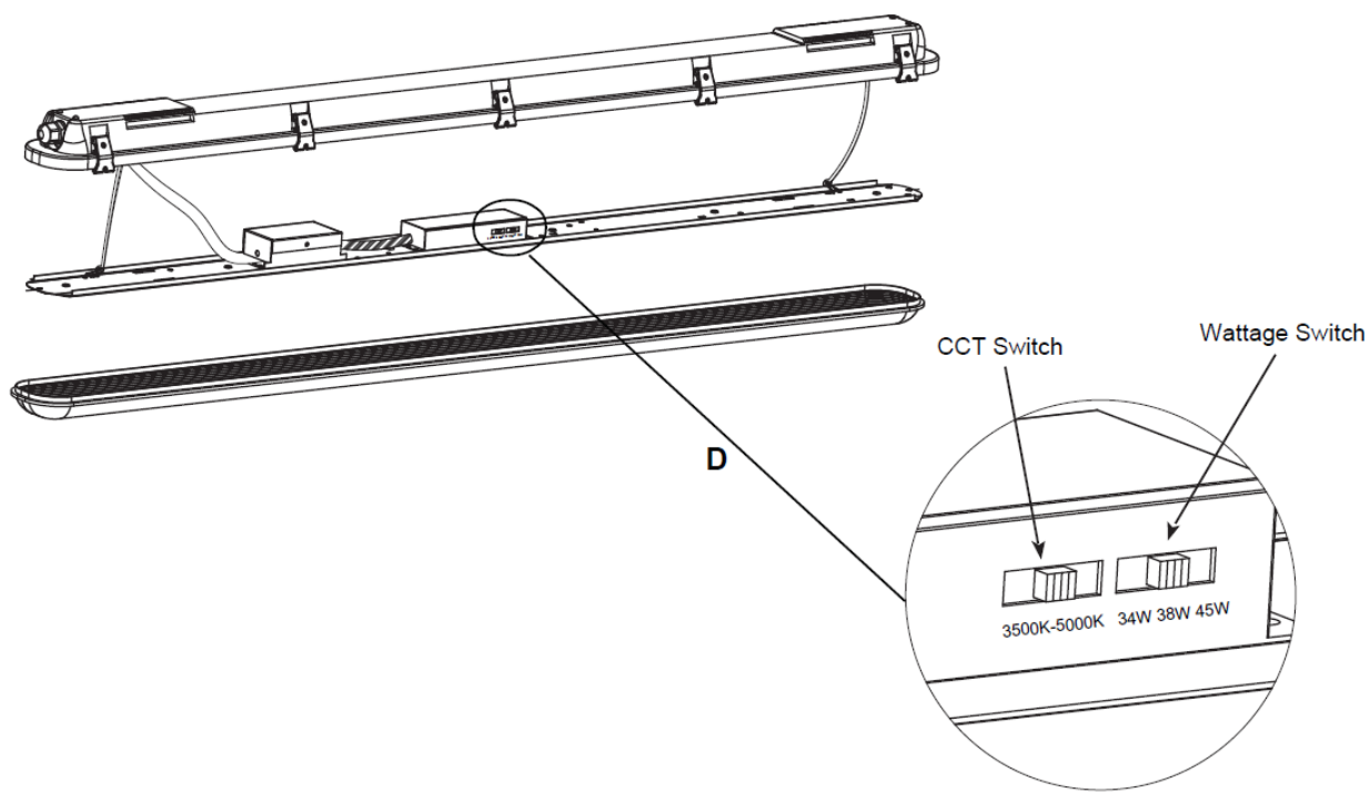
Color Temperature Switch and Wattage Switch Locations
