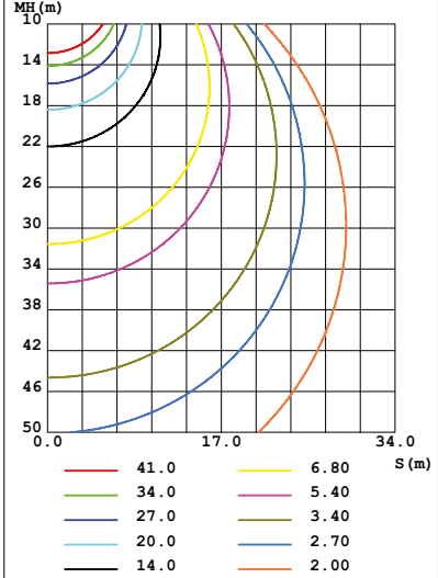
C0 PLANE ISOLUX DIAGRAM (UNIT:lx)
