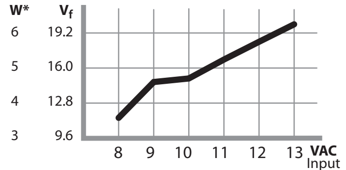
Voltage Input vs. Forward Voltage Output
