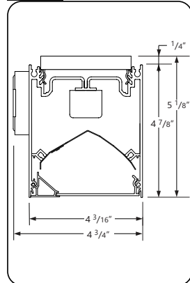
ASO Asymmetric with SO - Direct
