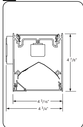
ASO Asymmetric with SO lens - Direct
