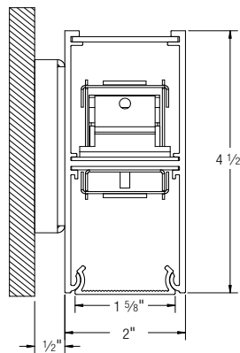
(W) Wall mount shown with snap-in-lens in the direct position & flexible white in the indirect position
