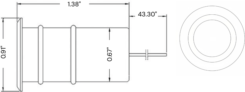
Aluminum Sleeve
