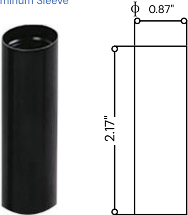
Aluminum Sleeve
