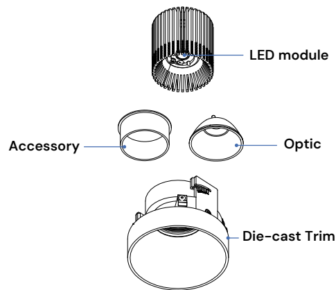
Round Trimless
