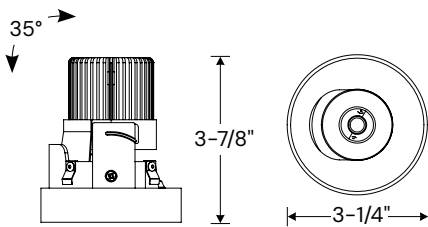
Round Adjustable Slot
