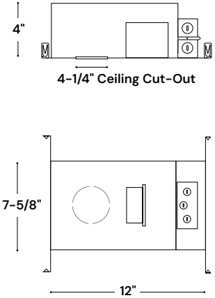
IC / CH - Housing
