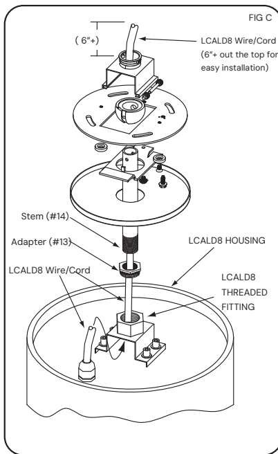
12301-8 with stem installation
