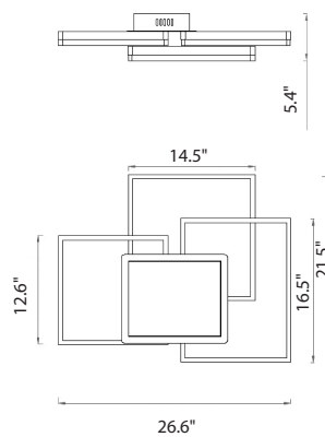
3 Tier Dimensions
