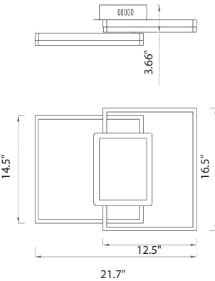
2 Tier Dimensions
