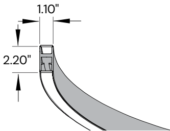
Cross Section
