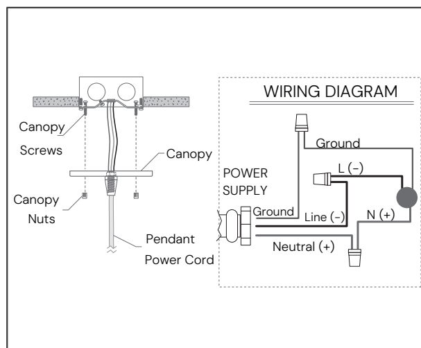
2 Make wire connections
