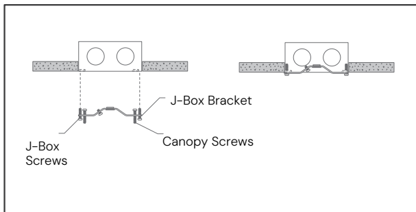
1 Install J-Box bracket
