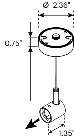
2" Angled Connector Left C2L
