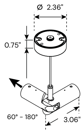
2" Angled Connector Right C2R
