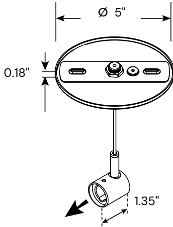
5" Angled Connector Left C5L
