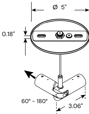
5" Angled Connector Right C5R
