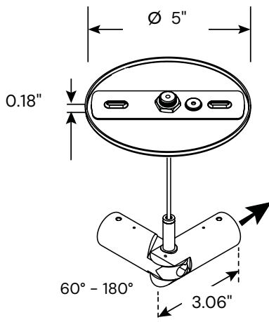
5" Angled Connector Right C5R
