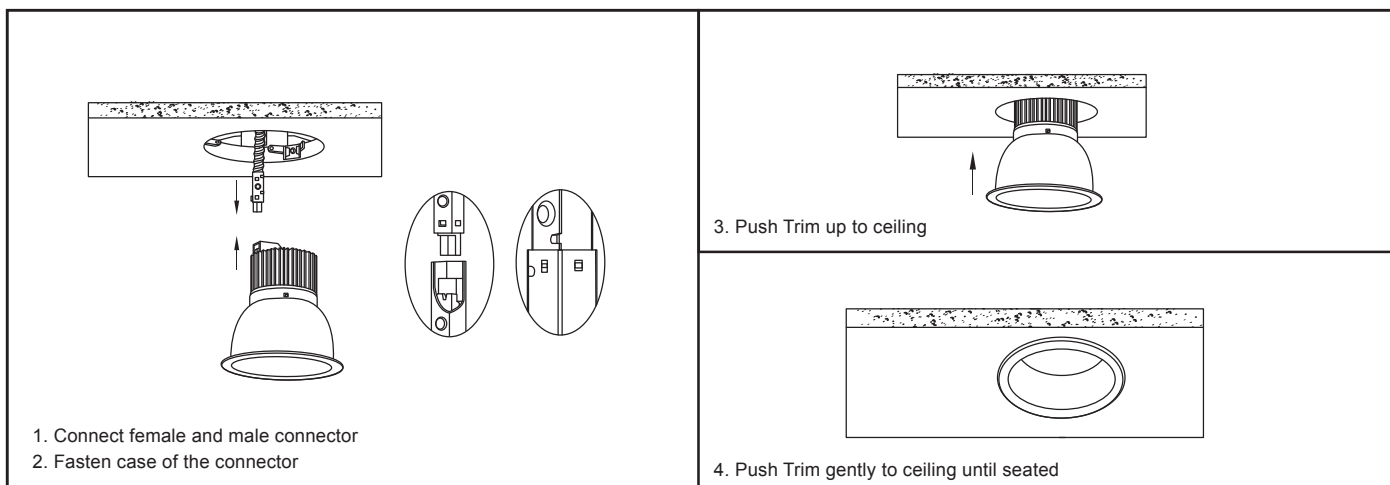
Push - In connector
