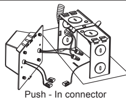
Push - In connector
